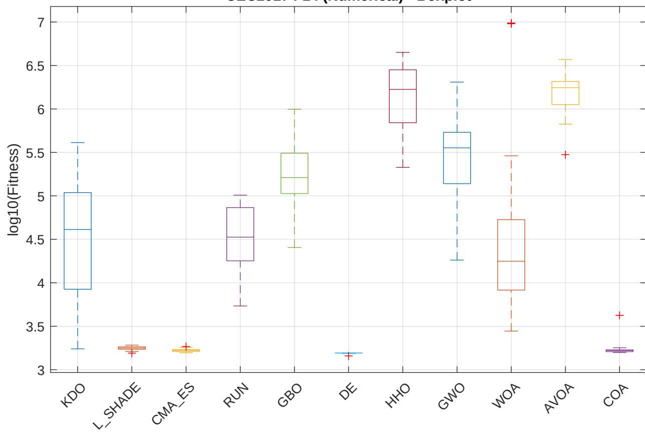
CEC2017 F14 (Numerical) - Boxplot
